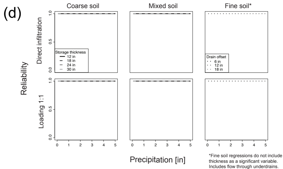
Paved green infrastructure: 80% reduction, 24 hour duration
