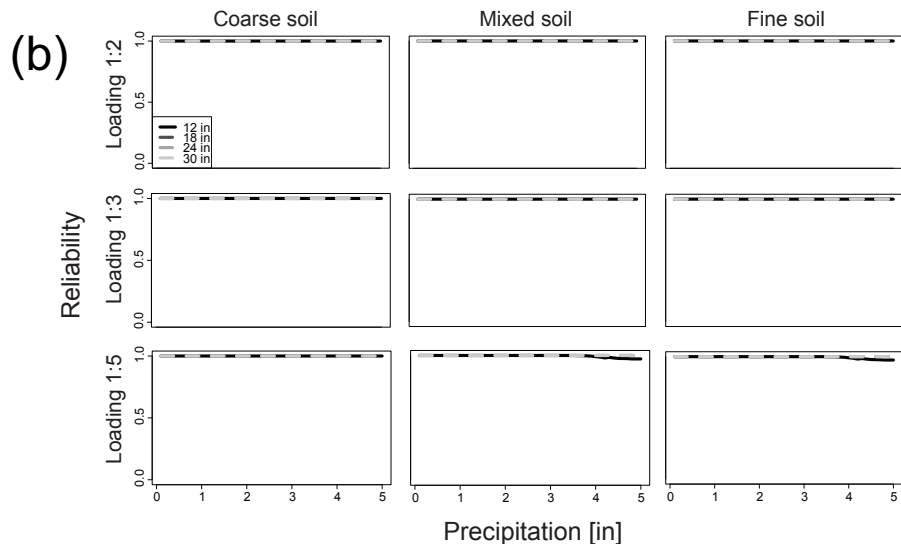
Planted green infrastructure: 80% reduction, 24 hour duration
