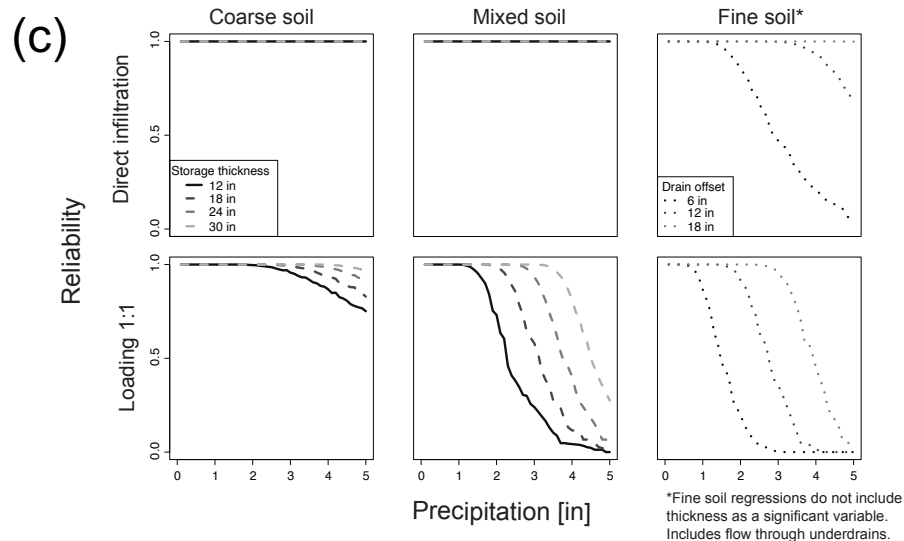
Paved green infrastructure: 80% reduction, 2 hour duration
